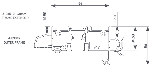
Standard open out outer frame with trickle vent
