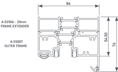
Standard outer frame with 20mm extender
