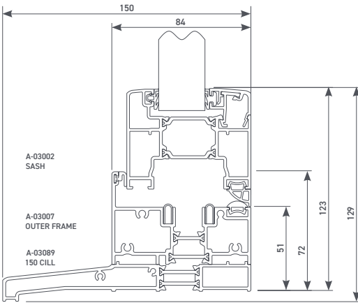
150mm cill with outer frame & sash profile - Open in
