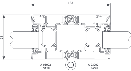
Sash to sash
